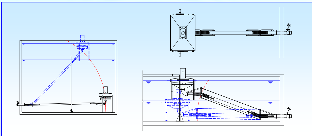
Mooring with hinged discharge system and vertical guiding post on the bottom of the basin
