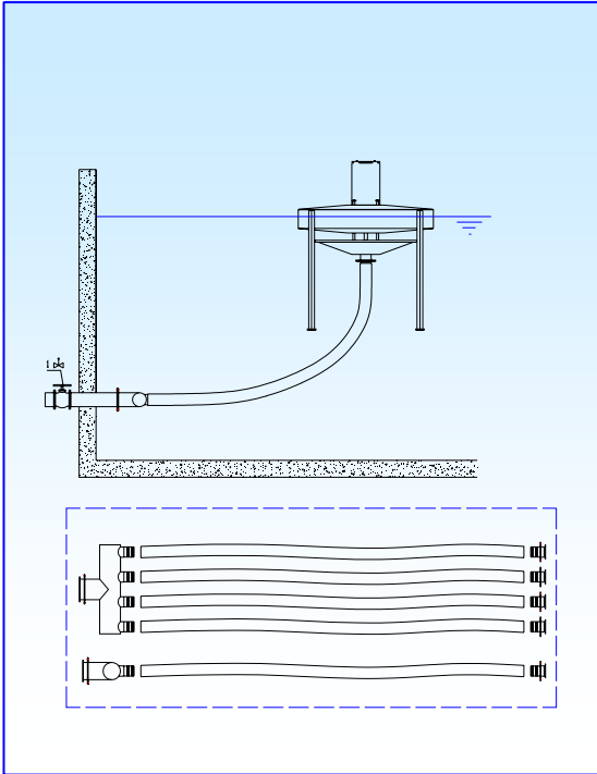
Flexible hose up to DN150 or Multiple flexible hoses (DN150) with collector up to DN300
