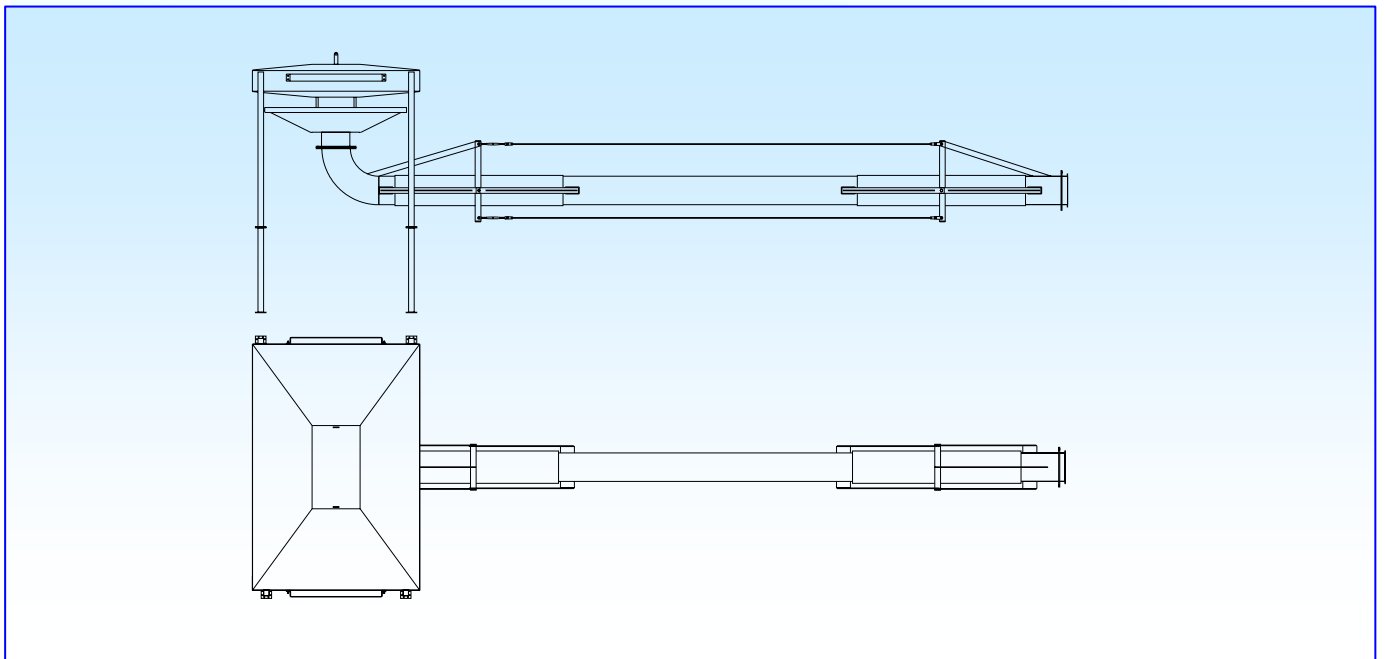
Hinged discharge system up to DN450
