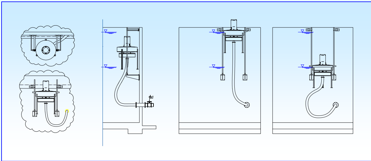
Mooring with vertical guiding posts on the side of the basin
