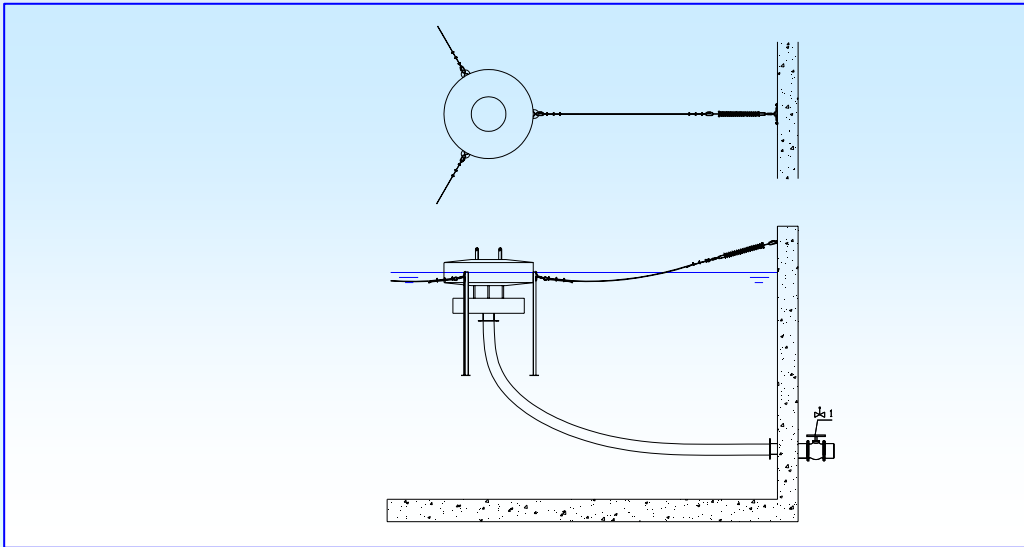
Mooring with cables and compression springs
