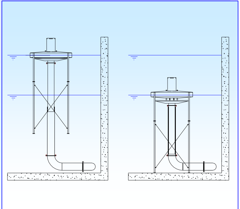
Telescopic discharge pipe up to DN450
